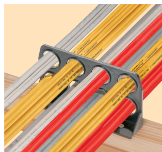
CA8 on wood joist power (NM) cables
