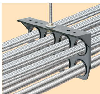
CA8L on threaded rod, power (MC) cables
