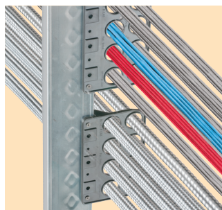
(2) CA8L on steel stud power & low voltage cables
